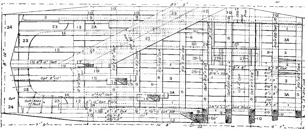
Fig. 411. Half Plan and Half Horizontal Section.
